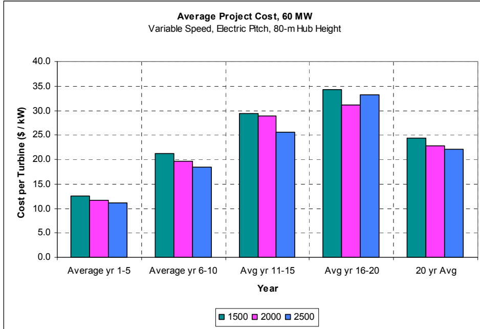
Figure 14. Average cost per kW, 60-MW project
